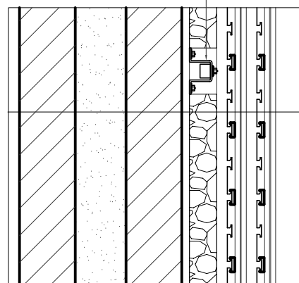
REMAK® G50Q WALL VIBRATION ABSORBER
