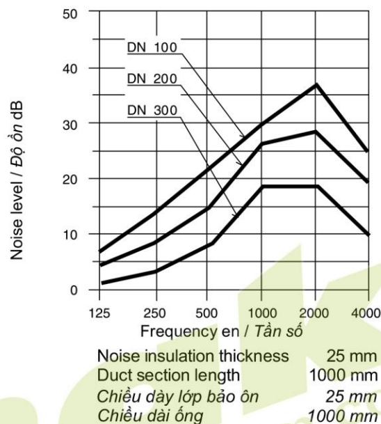
Figure 3: noise level for Insulated flexible duct
